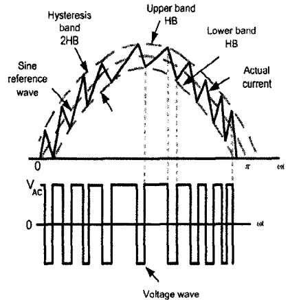
Fig. 4. Voltage Wave Control Input Signal Generation
